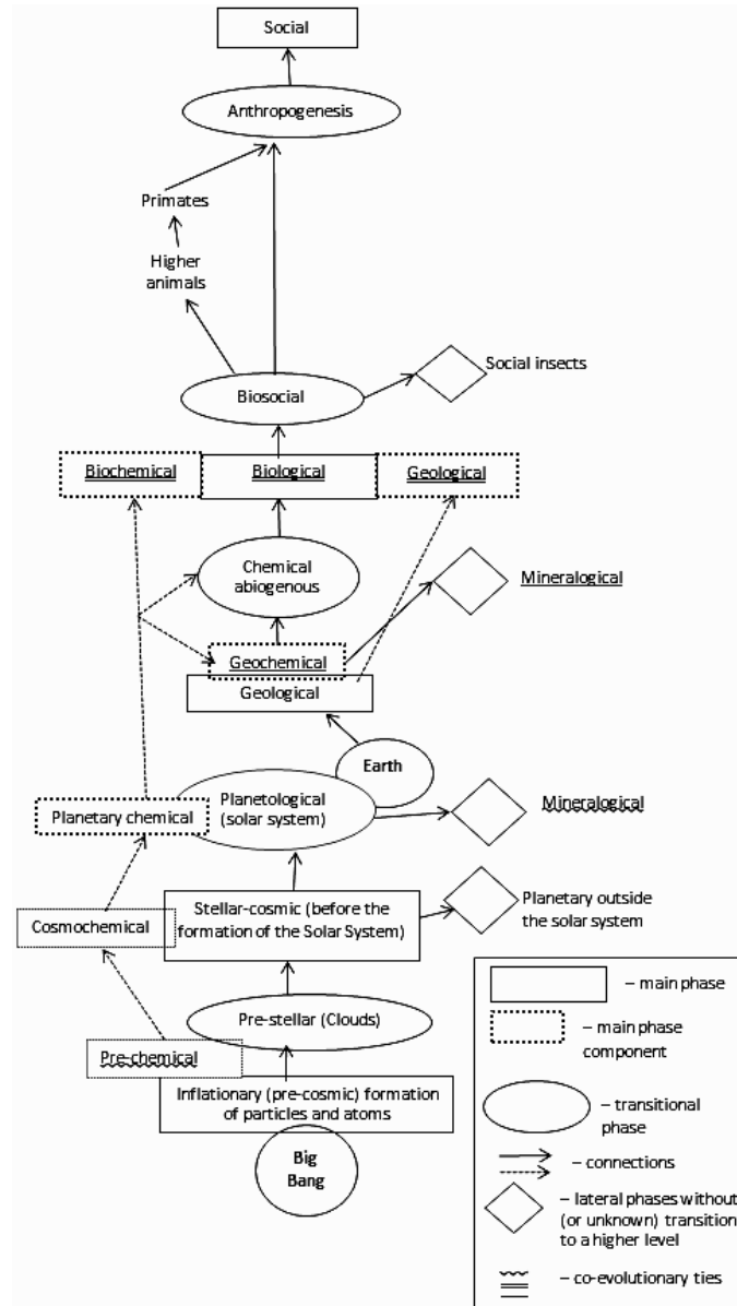
Fig. 1. Phases and lines of Universal evolution
