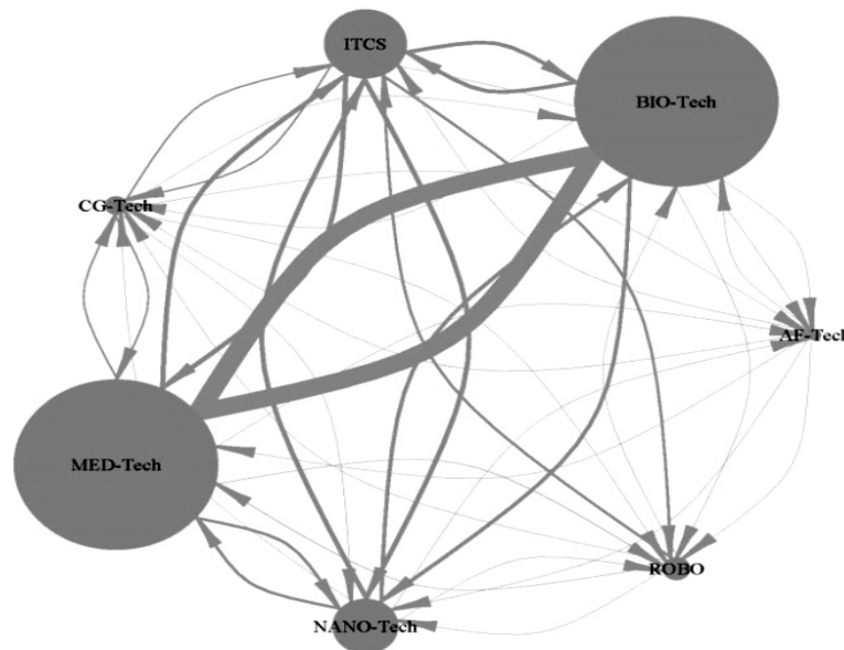
Fig. 2. The relationship between citation frequency in scientific publications and the technologies forming MANBRIC, according to the Web of Science, 2010–2015
