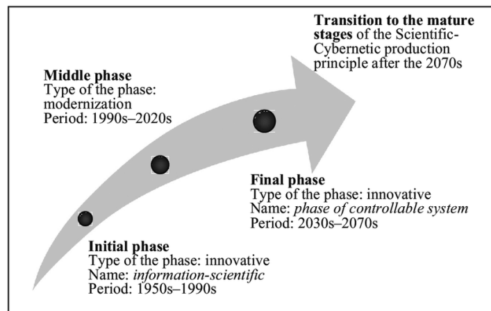
Fig. 1. The phases of the Cybernetic Revolution
