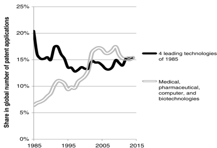
Fig. 3. Dynamics of the global combined share of four technologies with the highest share of patent applications in 1985 (electrical machinery, measurement, machine tools, and other special machines) in comparison with the dynamics of the global combined share of patent applications in four top categories (medical, pharmaceutical, computer, and biotechnologies), 1985–2014
